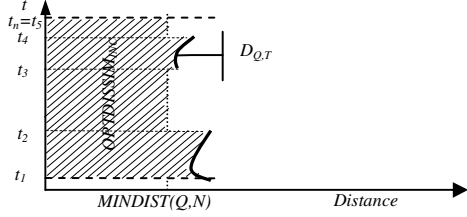
Figure 6. OPTDISSIM_{INC} definition
