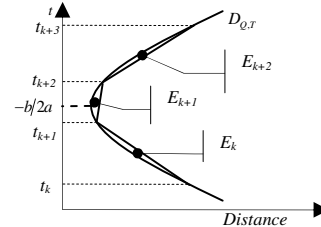
Figure 2. Trapezoid approximation
