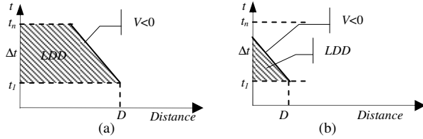
Figure 3. LDD definition
