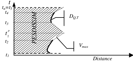
Figure 5. PESDISSIM definition
