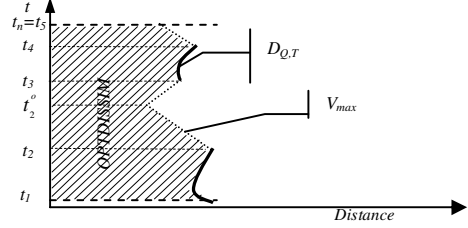
Figure 4. OPTDISSIM definition
