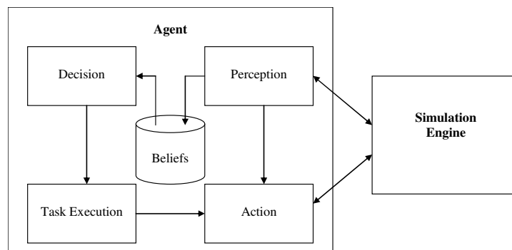
Figure 2: Agent Architecture
