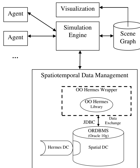
Figure 1: Virtual Environment Architecture
