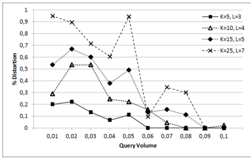
Figure 18: Distortion vs. query size w.r.t. the value of K – TrajFaker
