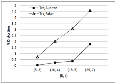
Figure 14: Distortion by range queries w.r.t. K, L
