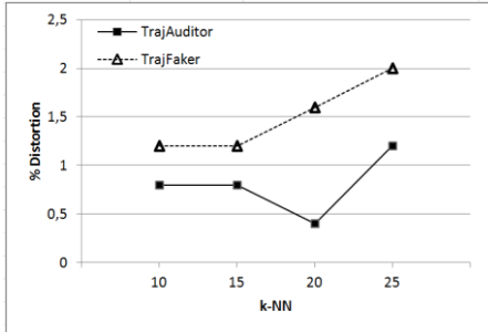
Figure 15: Distortion by kNN queries w.r.t k (K = 5)
