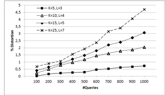
Figure 17: Distortion over time w.r.t. the value of K - TrajFaker
